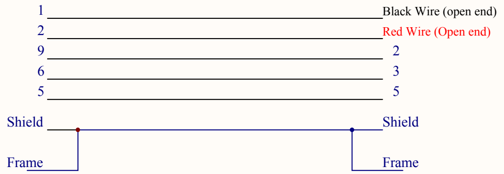
DB9 Female Plug (solder pin) with casing
